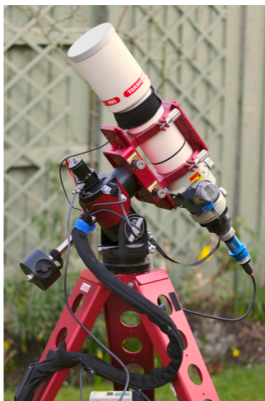
The Pegasus Power box makes for a simple one-wire connection from the mount to the ground (above). Below that, a conventional setup requires a cable bundle to prevent snagging and improve tracking consistency.
